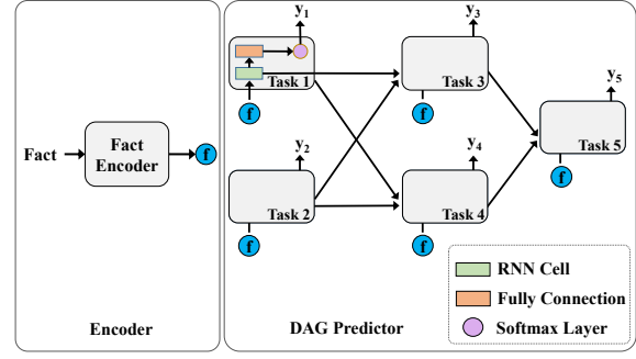
Figure 2: The framework of TOPJUDGE.
