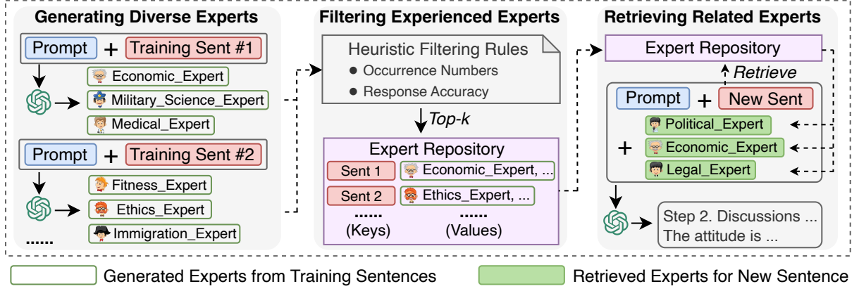
Figure 3: The overall pipeline of our DEEM method. We first use the prompt and training sentences to generate diverse experts (§ 3.1). Then we filter experienced experts according to their occurrence numbers and performance (§ 3.2). Finally, we build the sentence-expert pairs and retrieve the experienced experts for each new sentence (§ 3.3).
