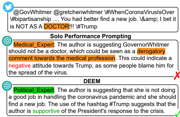
Figure 7: Example of solo performance prompting (Wang et al., 2023d) with generated experts (Middle) and our method with filtered experienced experts through retrieval (Bottom).
