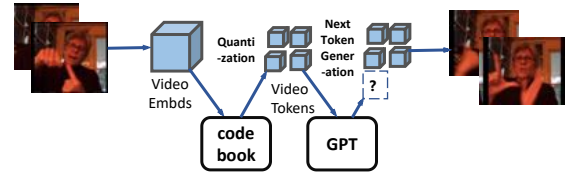
Figure 1: A figure describing sign video reconstruction module. This module is responsible for reconstructing the original video from the downsampled discrete latent representations of raw video data. In the quantization stage, the module transforms the video embeddings into discrete video tokens using a codebook. These video tokens are then input into GPT to generate the next visual token.
