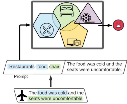
Figure 1: Text classification with PADA . Colored text signifies relation to a specific source domain. PADA first generates the domain name, followed by a set of DRFs related to the input example. Then it uses the prompt to predict the task label.
