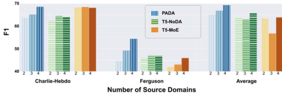
Figure 6: Performance on the Rumour Detection task by the number of source domains the model was trained on. Darker hues represent a larger number of source domains.
