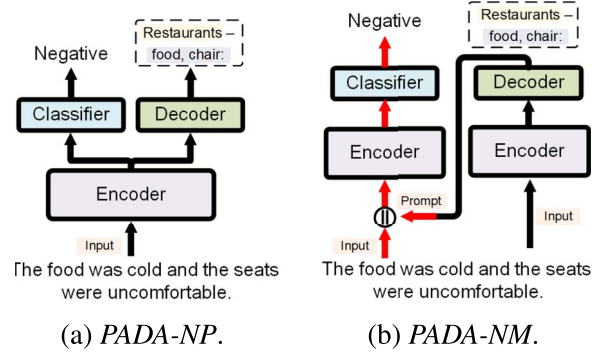
Figure 3: PADA ablation models: (a) PADA-NP , which follows a multi-task training protocol, but does not condition its prediction on the generated prompt; (b) PADA-NM , which separately trains a prompt generation model ( \rightarrow ) and a prompted task prediction model ( \rightarrow ).
