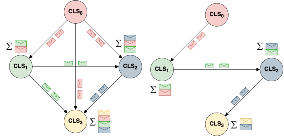
Figure 2: Node Representation Learning for a document with four sentences in single-layer GNN. Left: Semi-Complete Structure, Right: Linear Structure. During training, the sentence representation ( CLS_i ) are enriched using appropriate message passing techniques from the connected 1-hop neighbors.
