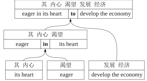
Figure 2: An example of function word insertion.
