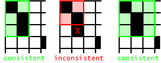
Figure 5: Definition of consistent word alignments: Words of an extracted phrase pair have to be aligned to each other and nothing else
