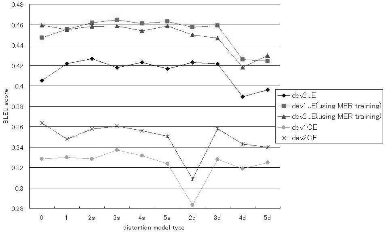
Figure 6: BLEU score of Japanese-English and Chinese-English translation with different distortion models
